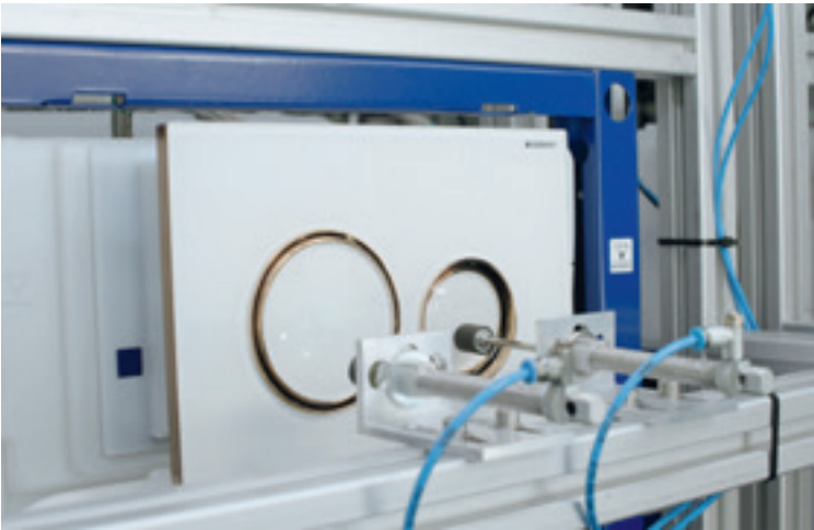
→ PRESSURE TEST The components for flush actuation must be able to withstand at least 200,000 actuations, corresponding to a service life of around 50 years.
