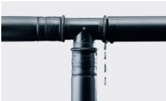
↑ Unpressed fittings can be reliably identified during a leak test.
