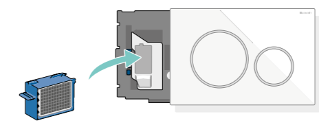
↑ The ceramic honeycomb filter is readily accessible behind the actuator plate.
